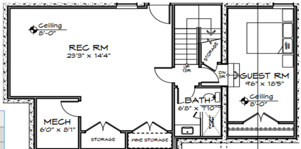
TBD TOVIDO LANE PROPOSED FLOOR PLAN
